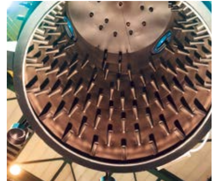
▲ Jet cooling with computer-optimized nozzle design results in 20 % higher cooling capacity.
