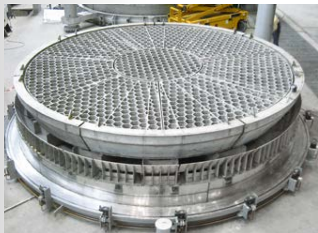
▲ Annealing base for nitrogen and hydrogen annealing with honeycomb grating and set of confusor/ diffuser parts made from heat-resistant material
